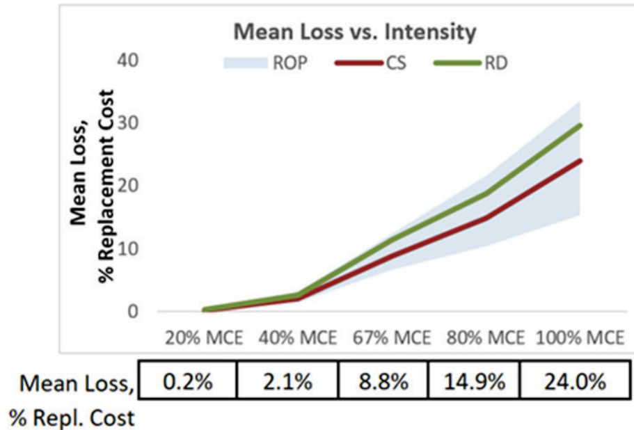
Figure C-3 Graph showing mean repair cost as a percentage of replacement cost on the User Interface tab.
