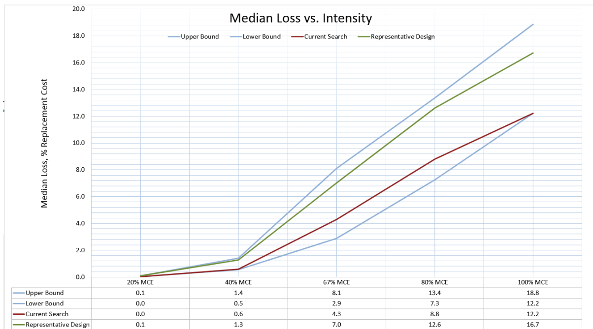
Figure C-4 Detailed plot of mean repair cost versus intensity.
